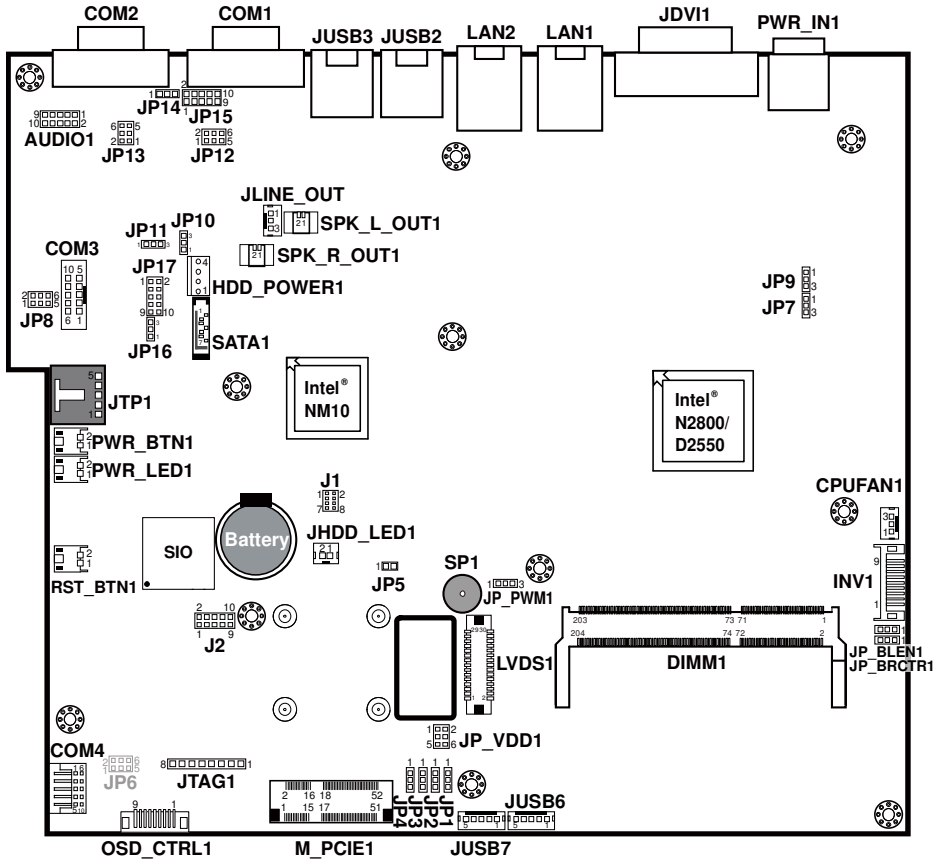
SP-6305/6307/6309 Connectors, Jumpers and Component Locations
