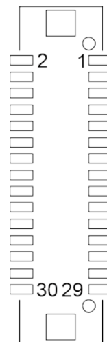
LVDS1
