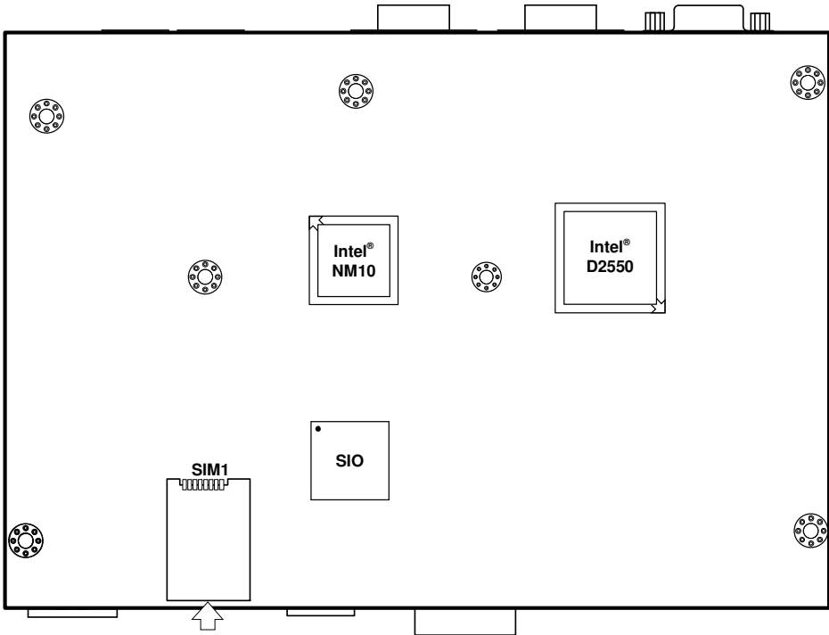
SP-6130/6132/6135/6138 Connectors, Jumpers and Components Locations - Rear
